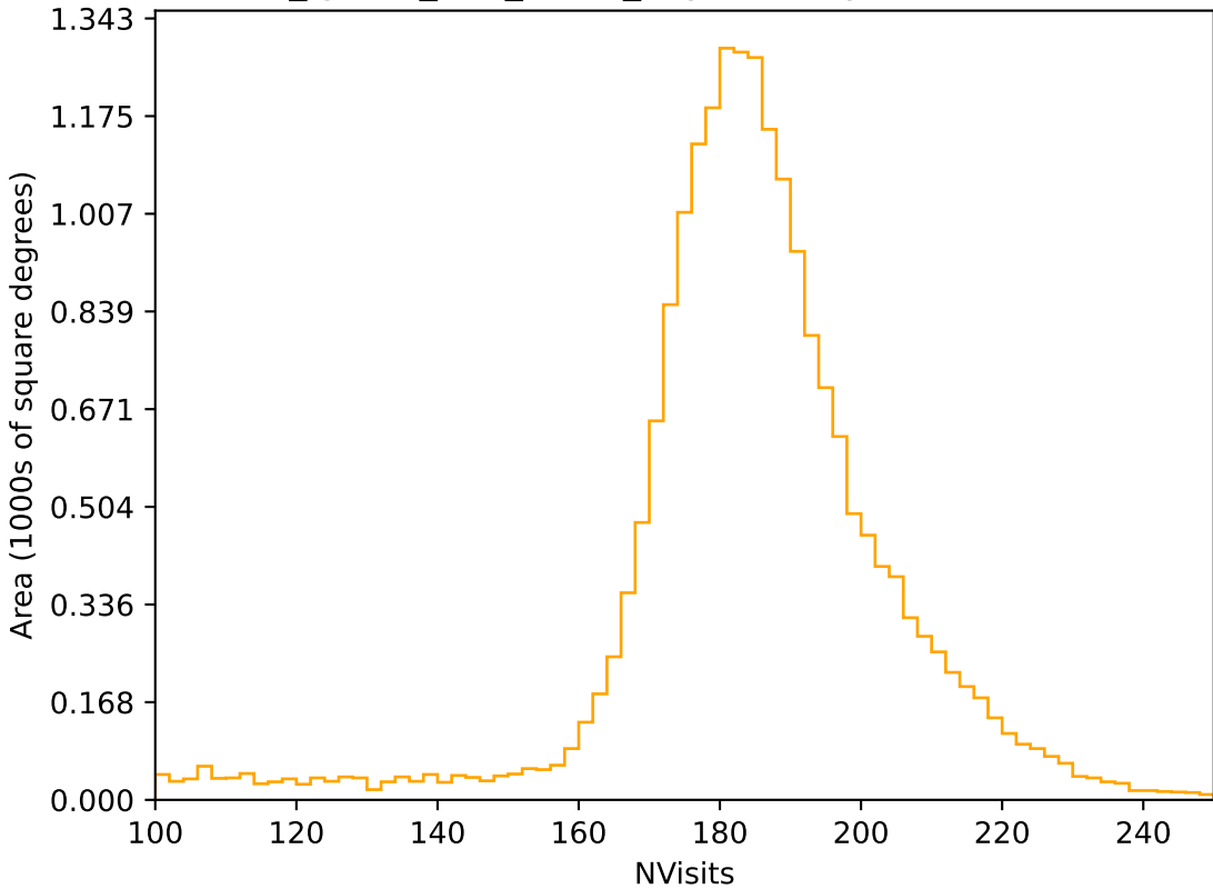
too_ignore_100_1v3.4_10yrs All sky r band: NVisits
