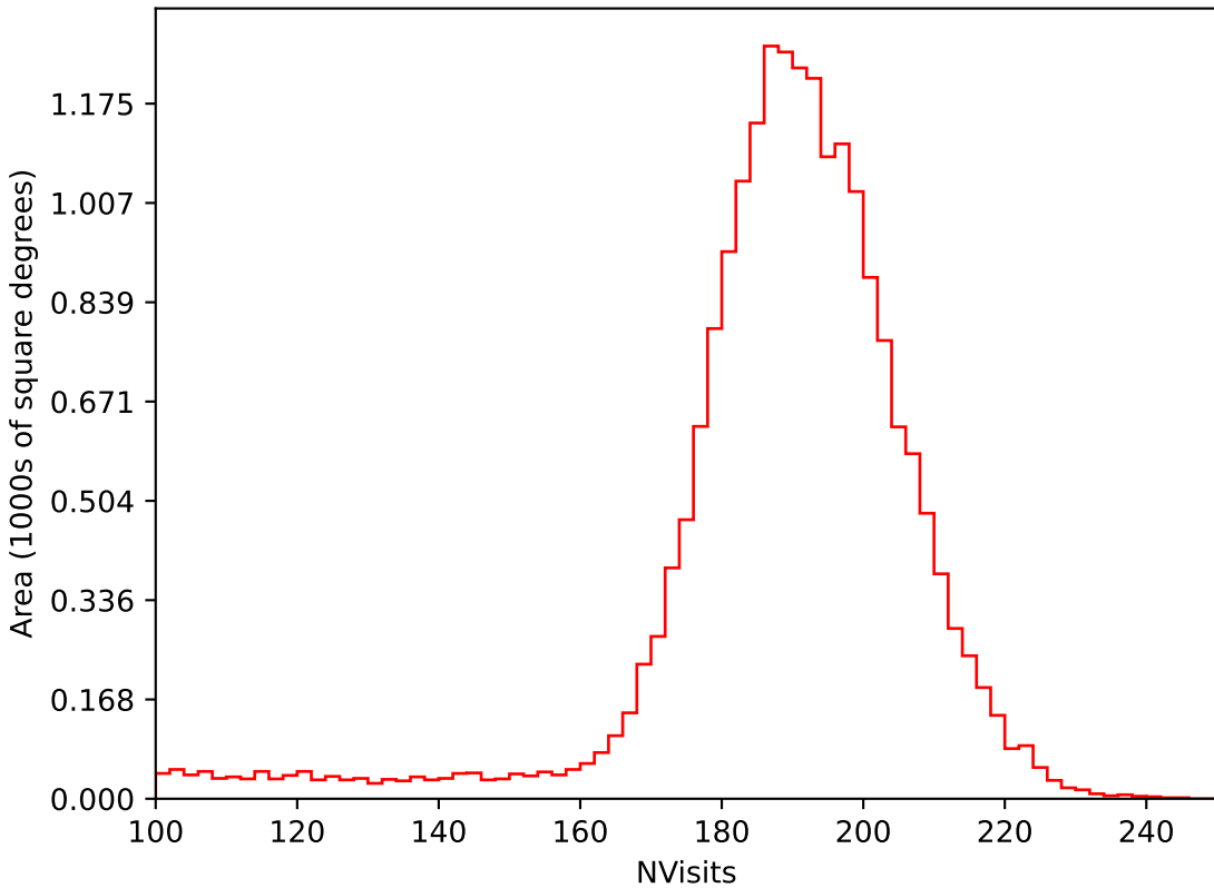
too_ignore_100_1v3.4_10yrs All sky i band: NVisits
