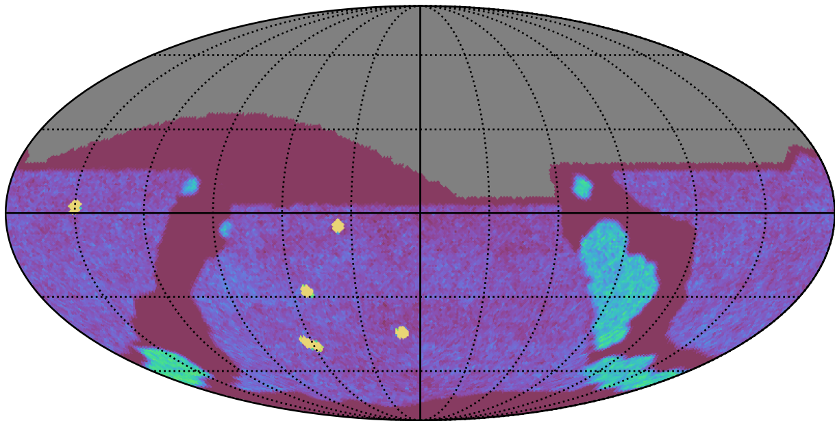
too_ignore_100_1v3.4_10yrs All sky g band: NVisits
