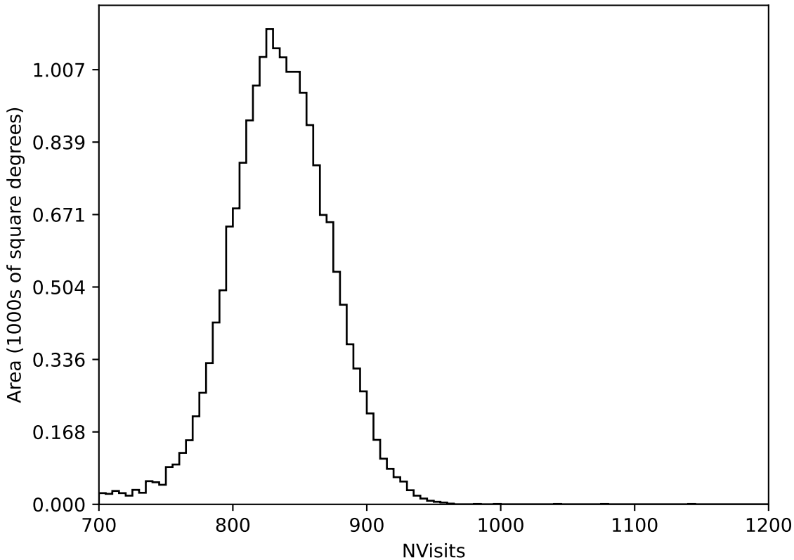
too_ignore_100_1v3.4_10yrs All sky all bands: NVisits
