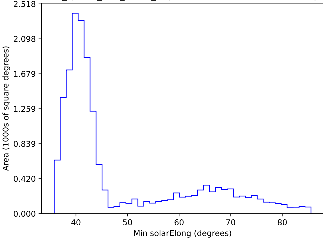
too_ignore_100_1v3.4_10yrs WFD z band: Min solarElong
