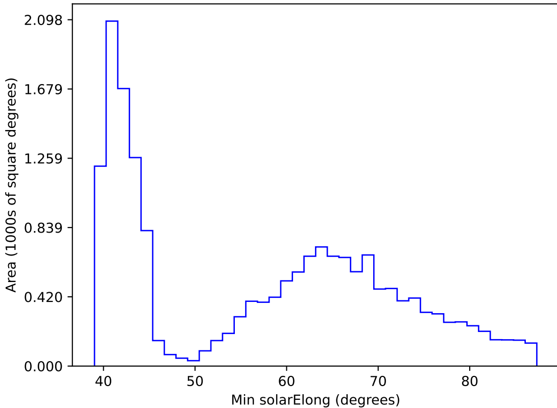
too_ignore_100_1v3.4_10yrs WFD r band: Min solarElong
