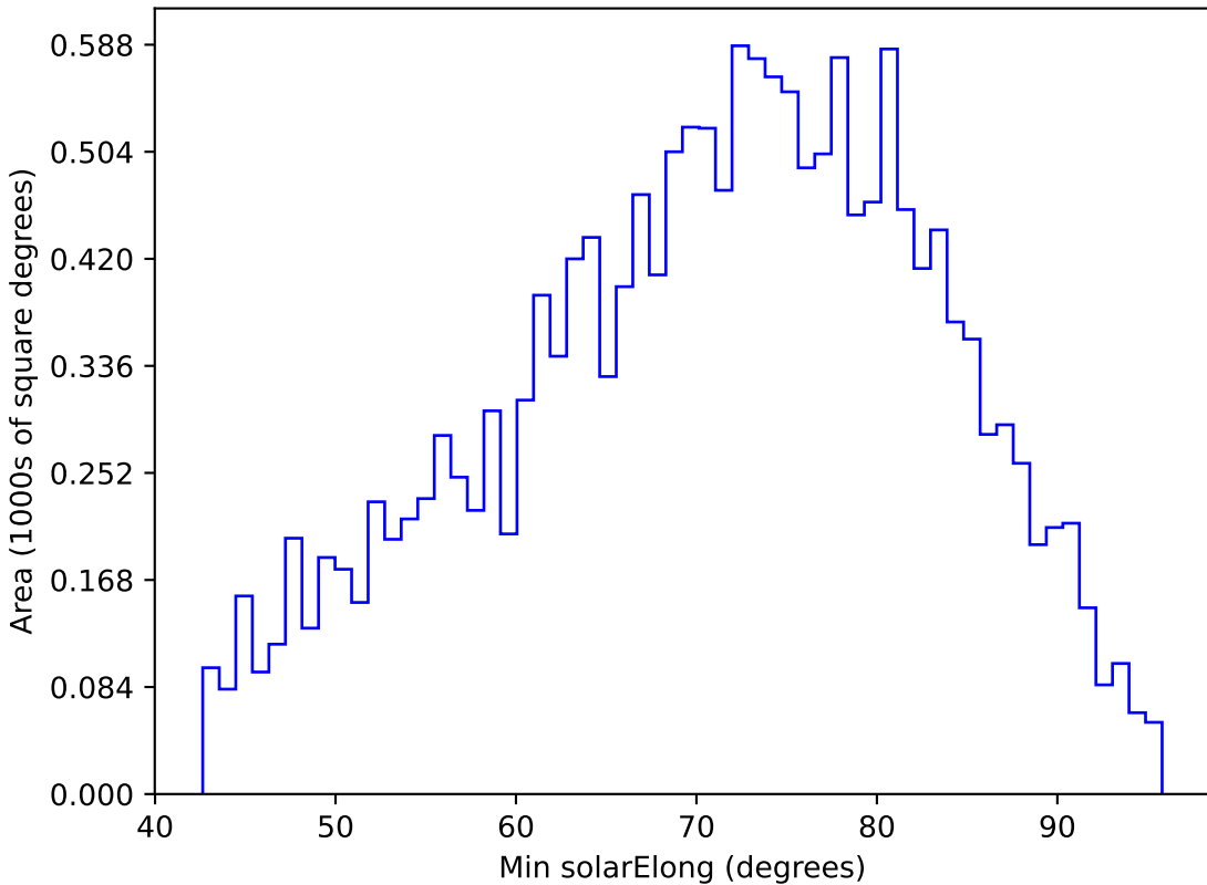
too_ignore_100_1v3.4_10yrs WFD g band: Min solarElong
