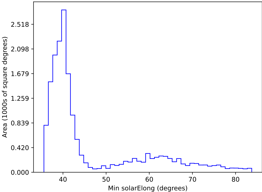
too_ignore_100_1v3.4_10yrs WFD all bands: Min solarElong
