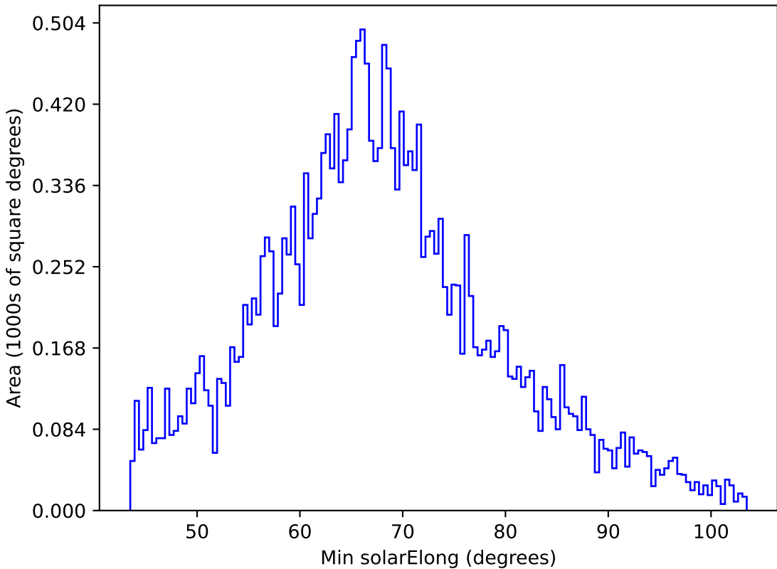
too_ignore_100_1v3.4_10yrs All sky y band: Min solarElong
