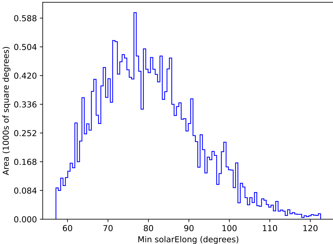
too_ignore_100_1v3.4_10yrs All sky u band: Min solarElong
