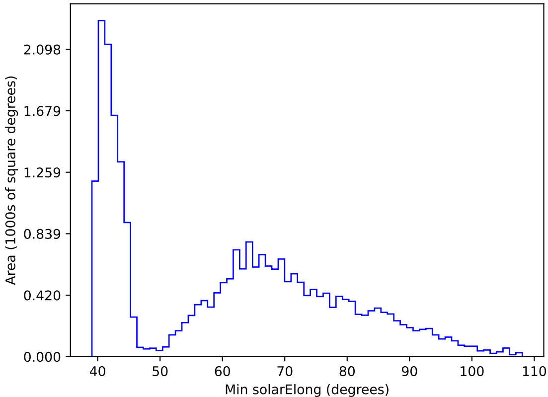
too_ignore_100_1v3.4_10yrs All sky r band: Min solarElong
