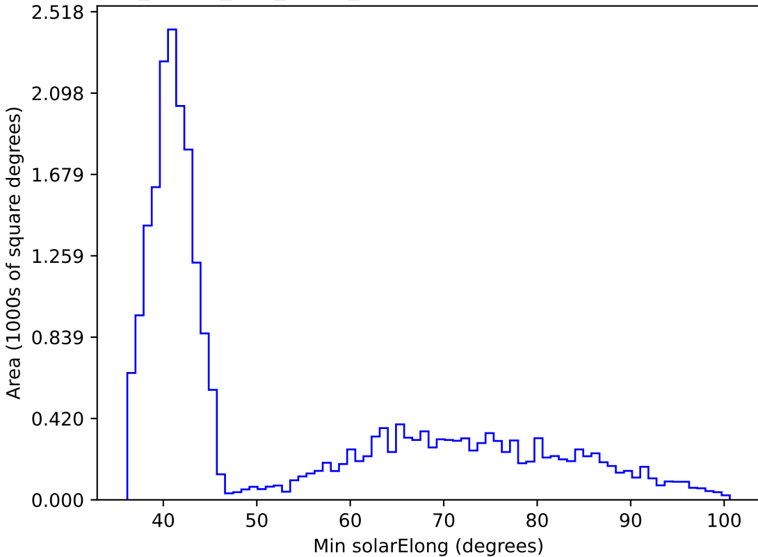
too_ignore_100_1v3.4_10yrs All sky i band: Min solarElong
