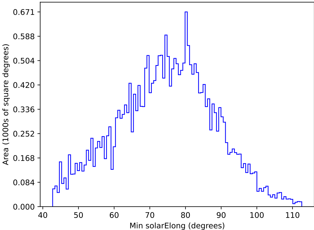
too_ignore_100_1v3.4_10yrs All sky g band: Min solarElong
