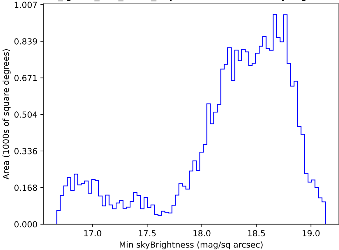
too_ignore_100_1v3.4_10yrs Yr 1 z band: Min skyBrightness
