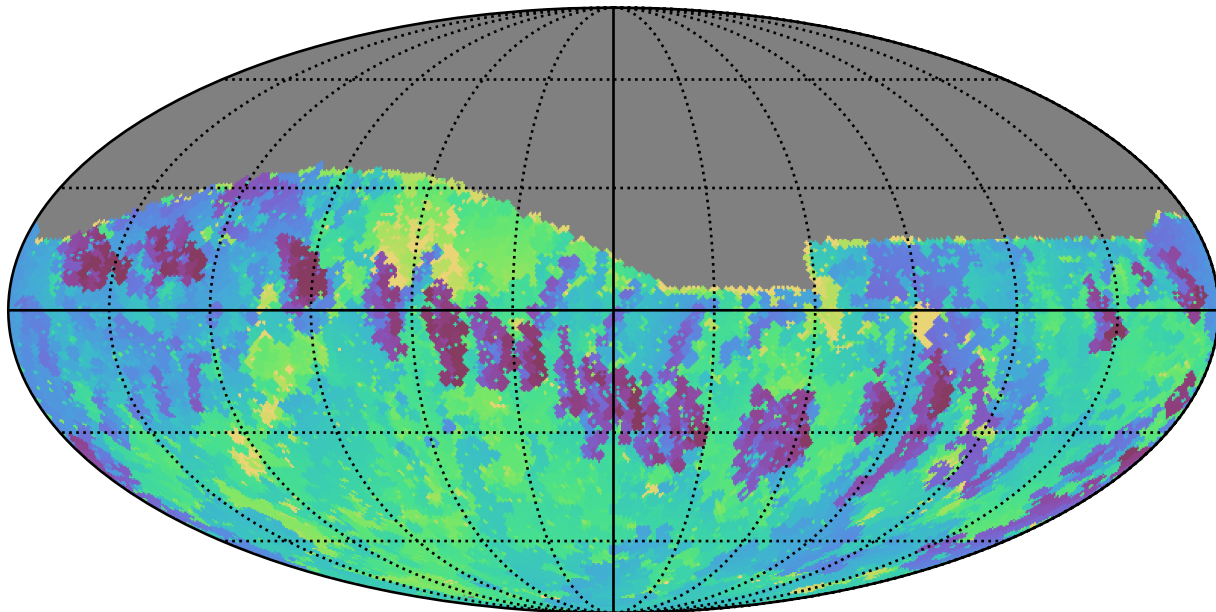
too_ignore_100_1v3.4_10yrs Yr 1 i band: Min skyBrightness
