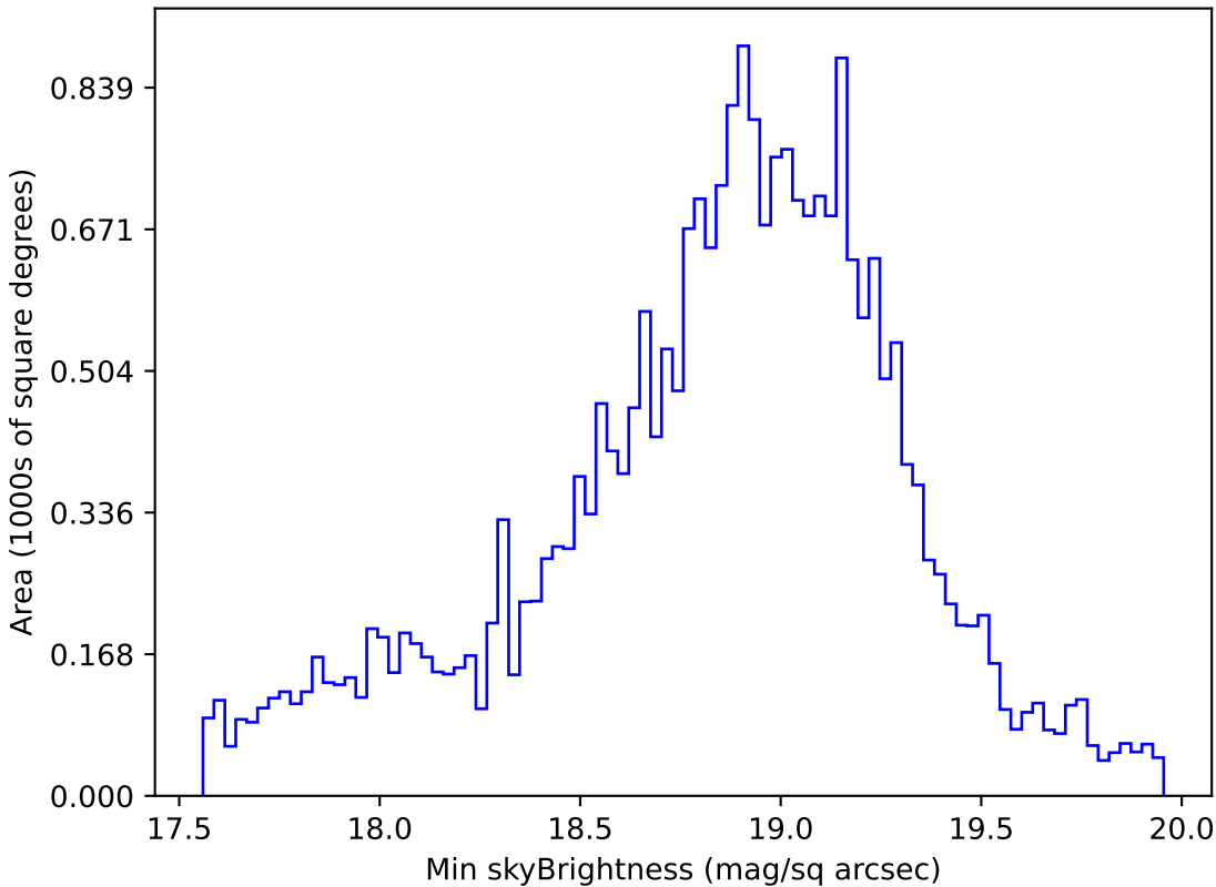
too_ignore_100_1v3.4_10yrs Yr 1 i band: Min skyBrightness
