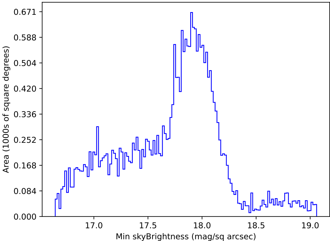
too_ignore_100_1v3.4_10yrs Yr 1 all bands: Min skyBrightness
