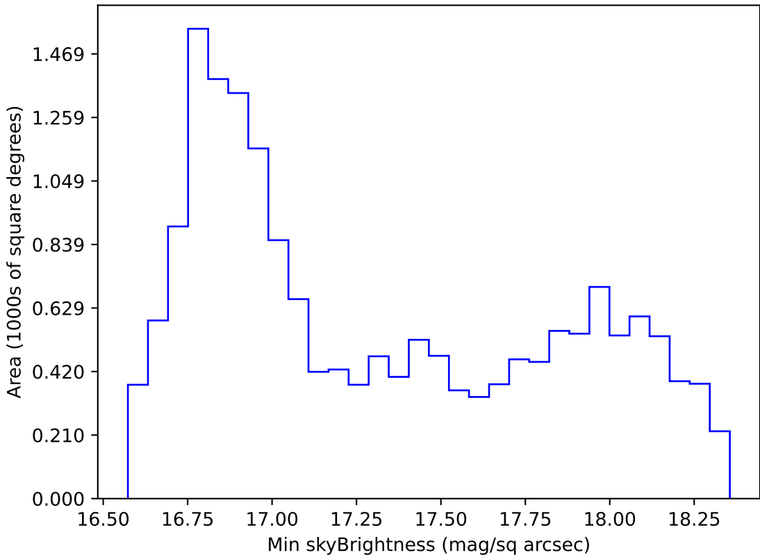
too_ignore_100_1v3.4_10yrs WFD z band: Min skyBrightness
