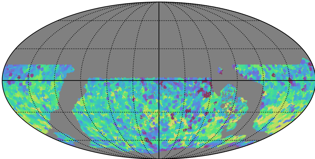
too_ignore_100_1v3.4_10yrs WFD y band: Min skyBrightness
