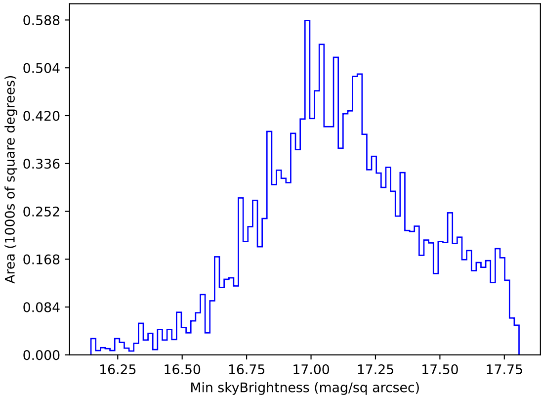
too_ignore_100_1v3.4_10yrs WFD y band: Min skyBrightness
