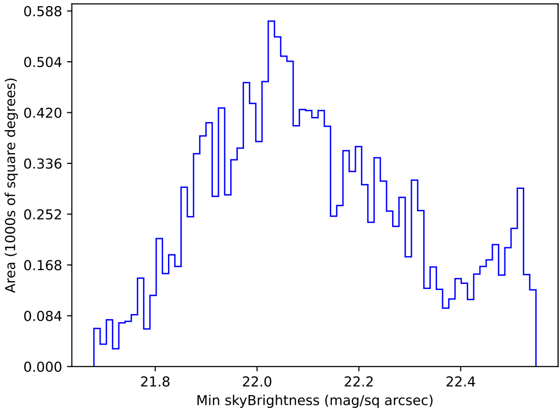
too_ignore_100_1v3.4_10yrs WFD u band: Min skyBrightness
