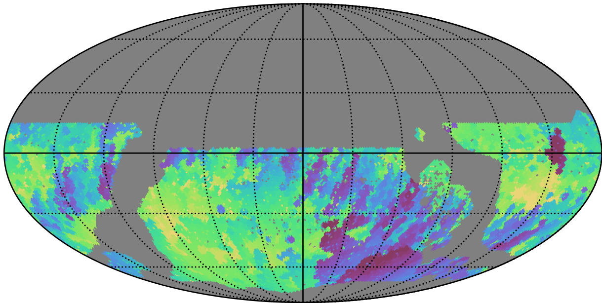
too_ignore_100_1v3.4_10yrs WFD r band: Min skyBrightness
