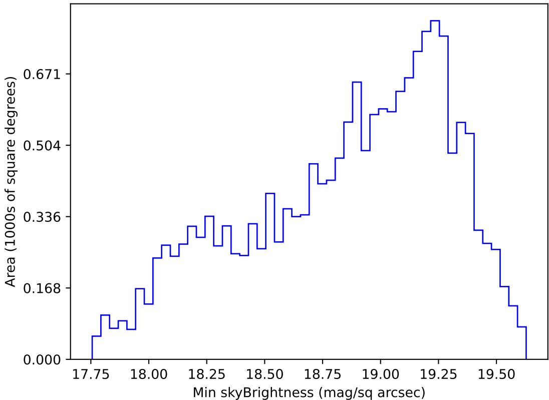
too_ignore_100_1v3.4_10yrs WFD r band: Min skyBrightness
