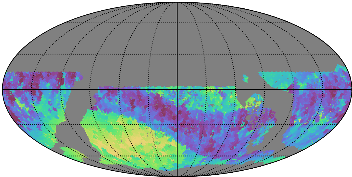
too_ignore_100_1v3.4_10yrs WFD i band: Min skyBrightness
