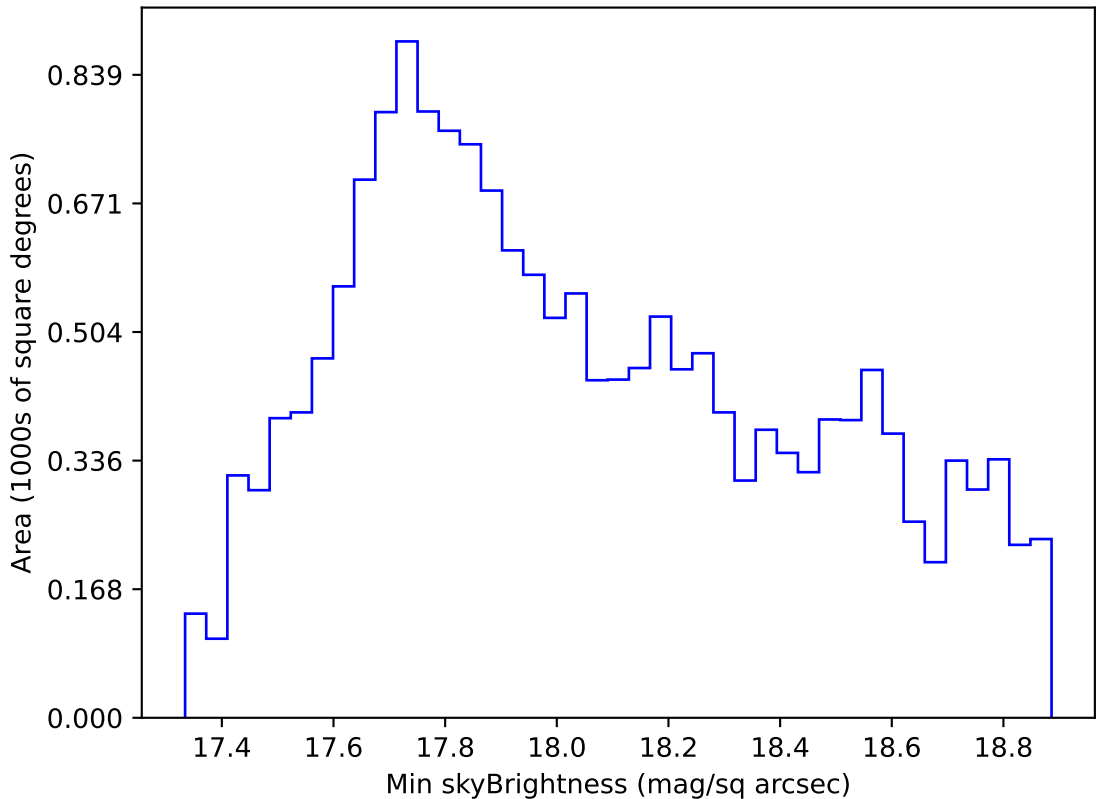
too_ignore_100_1v3.4_10yrs WFD i band: Min skyBrightness
