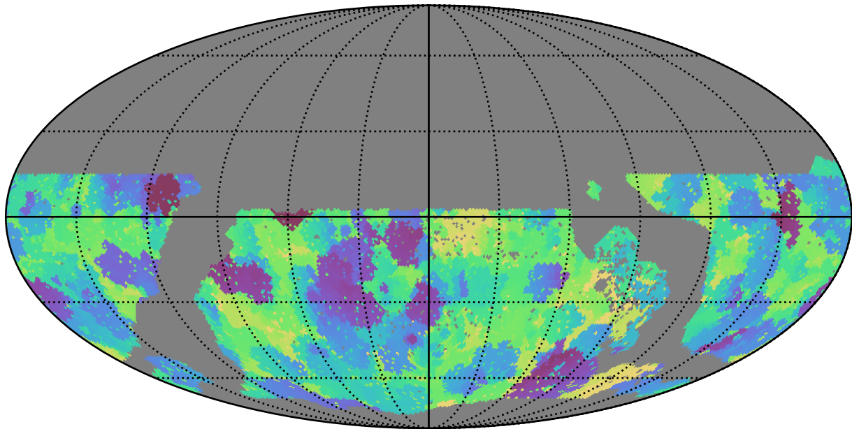
too_ignore_100_1v3.4_10yrs WFD g band: Min skyBrightness
