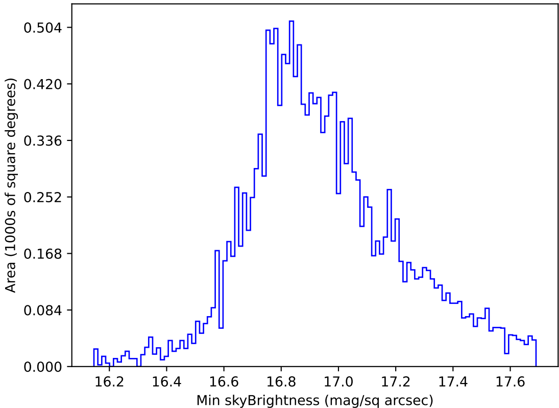
too_ignore_100_1v3.4_10yrs WFD all bands: Min skyBrightness
