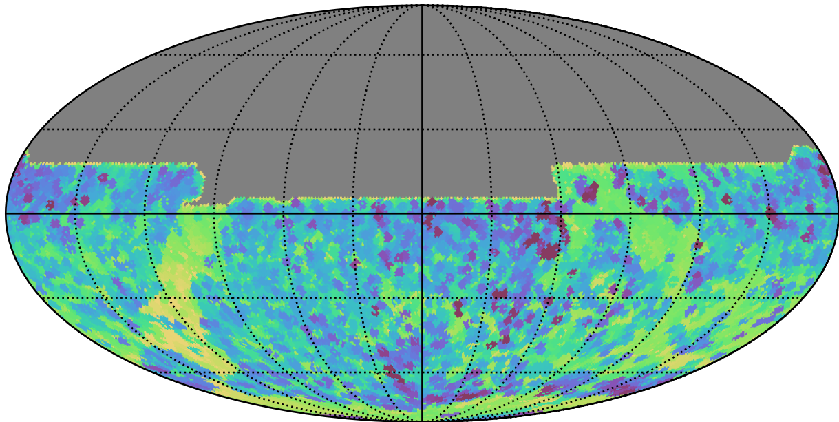
too_ignore_100_1v3.4_10yrs All sky y band: Min skyBrightness
