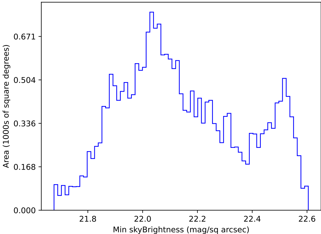
too_ignore_100_1v3.4_10yrs All sky u band: Min skyBrightness
