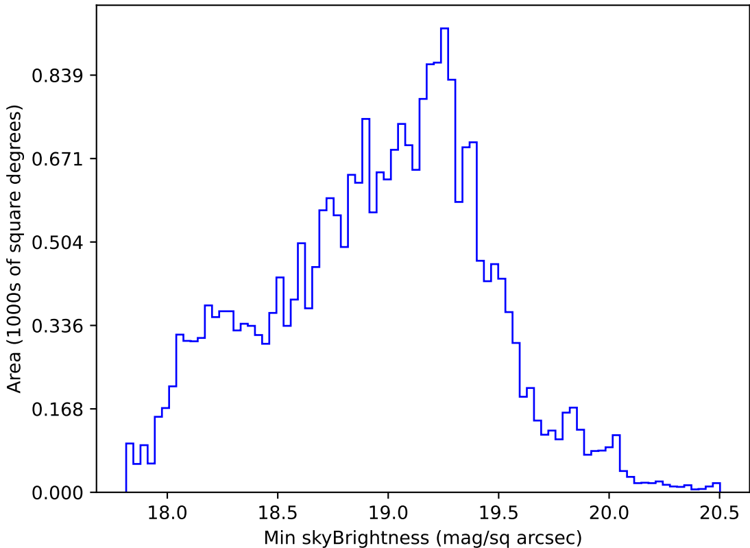
too_ignore_100_1v3.4_10yrs All sky r band: Min skyBrightness
