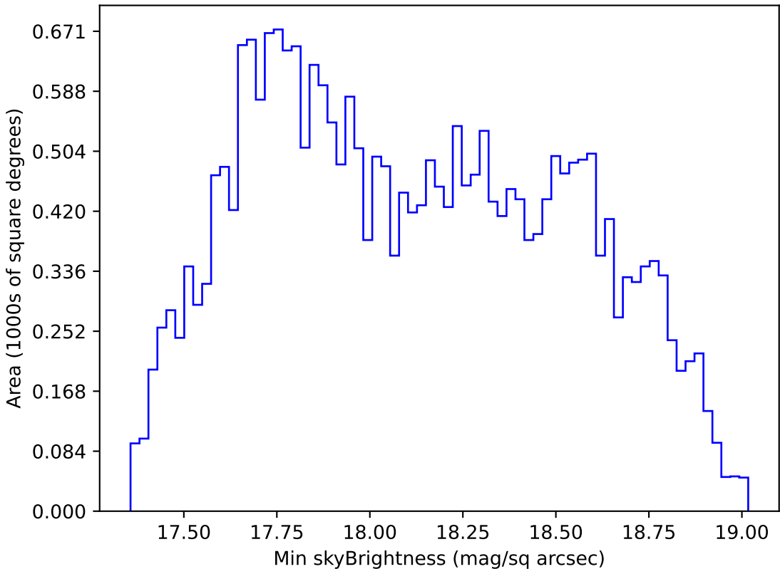
too_ignore_100_1v3.4_10yrs All sky i band: Min skyBrightness
