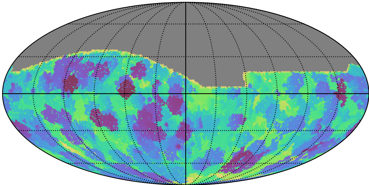
too_ignore_100_1v3.4_10yrs All sky g band: Min skyBrightness
