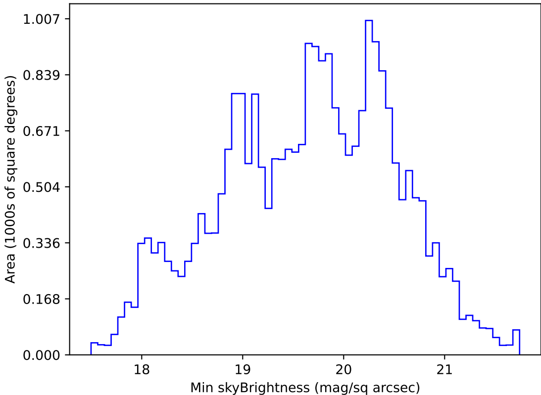
too_ignore_100_1v3.4_10yrs All sky g band: Min skyBrightness
