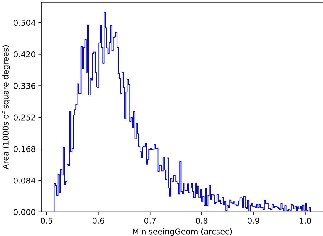
too_ignore_100_1v3.4_10yrs Yr 1 z band: Min seeingGeom
