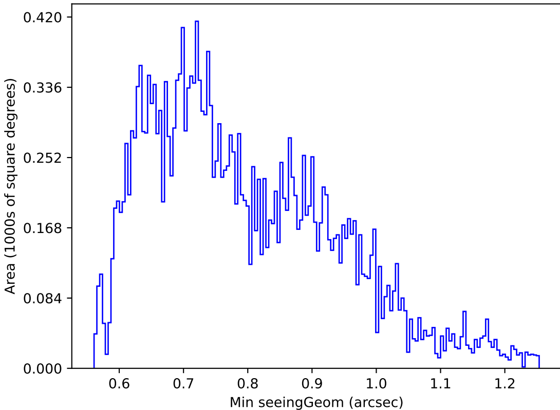
too_ignore_100_1v3.4_10yrs Yr 1 u band: Min seeingGeom
