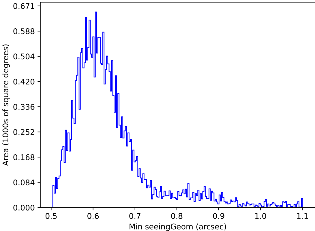
too_ignore_100_1v3.4_10yrs Yr 1 r band: Min seeingGeom
