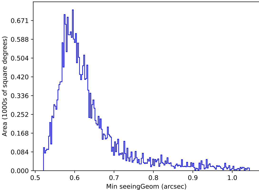
too_ignore_100_1v3.4_10yrs Yr 1 i band: Min seeingGeom
