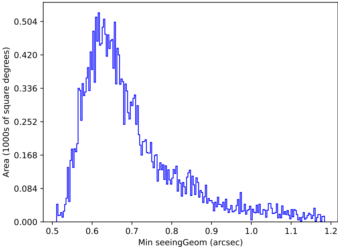
too_ignore_100_1v3.4_10yrs Yr 1 g band: Min seeingGeom
