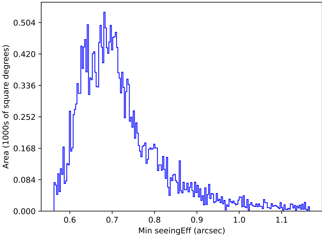
too_ignore_100_1v3.4_10yrs Yr 1 z band: Min seeingEff
