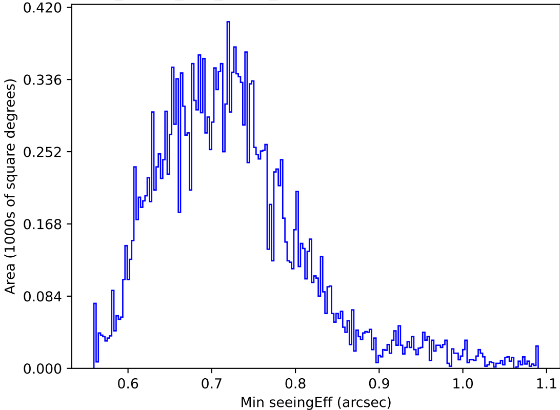
too_ignore_100_1v3.4_10yrs Yr 1 y band: Min seeingEff
