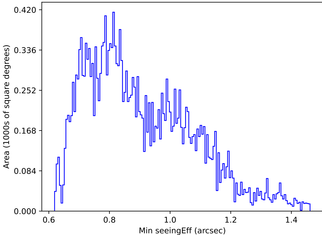
too_ignore_100_1v3.4_10yrs Yr 1 u band: Min seeingEff
