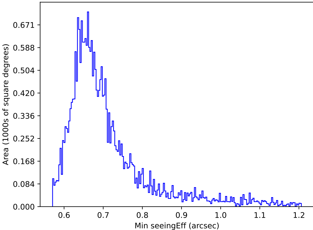
too_ignore_100_1v3.4_10yrs Yr 1 i band: Min seeingEff
