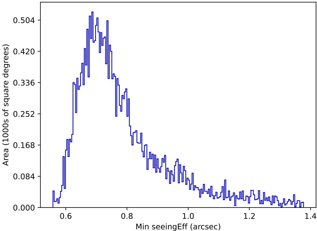
too_ignore_100_1v3.4_10yrs Yr 1 g band: Min seeingEff
