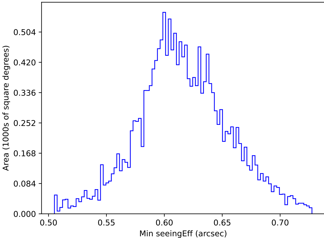
too_ignore_100_1v3.4_10yrs WFD z band: Min seeingEff
