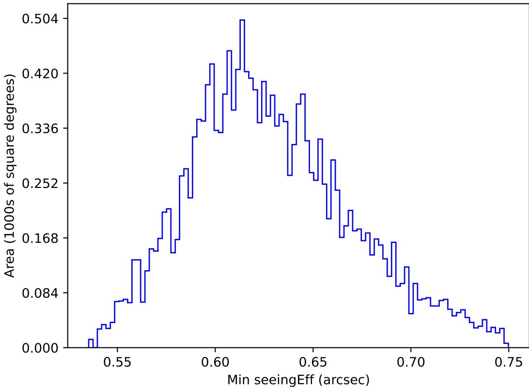
too_ignore_100_1v3.4_10yrs WFD y band: Min seeingEff
