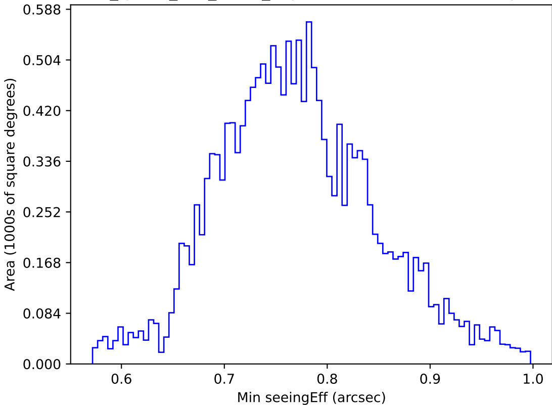
too_ignore_100_1v3.4_10yrs WFD u band: Min seeingEff
