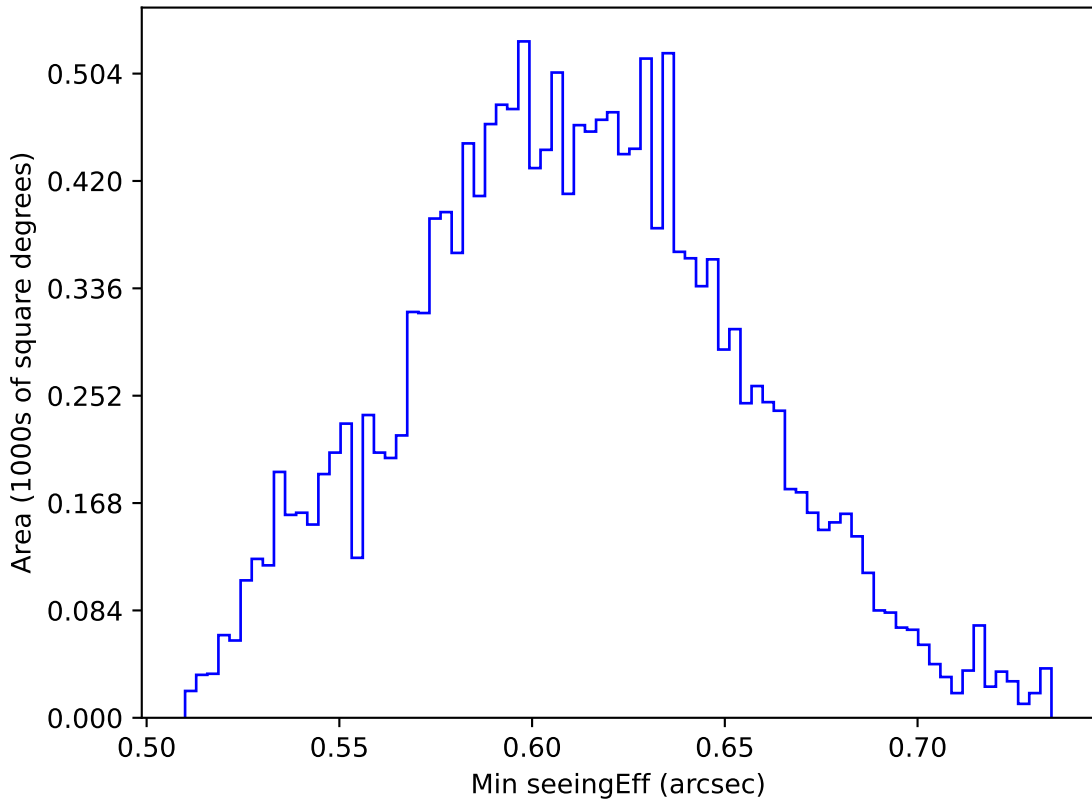
too_ignore_100_1v3.4_10yrs WFD r band: Min seeingEff
