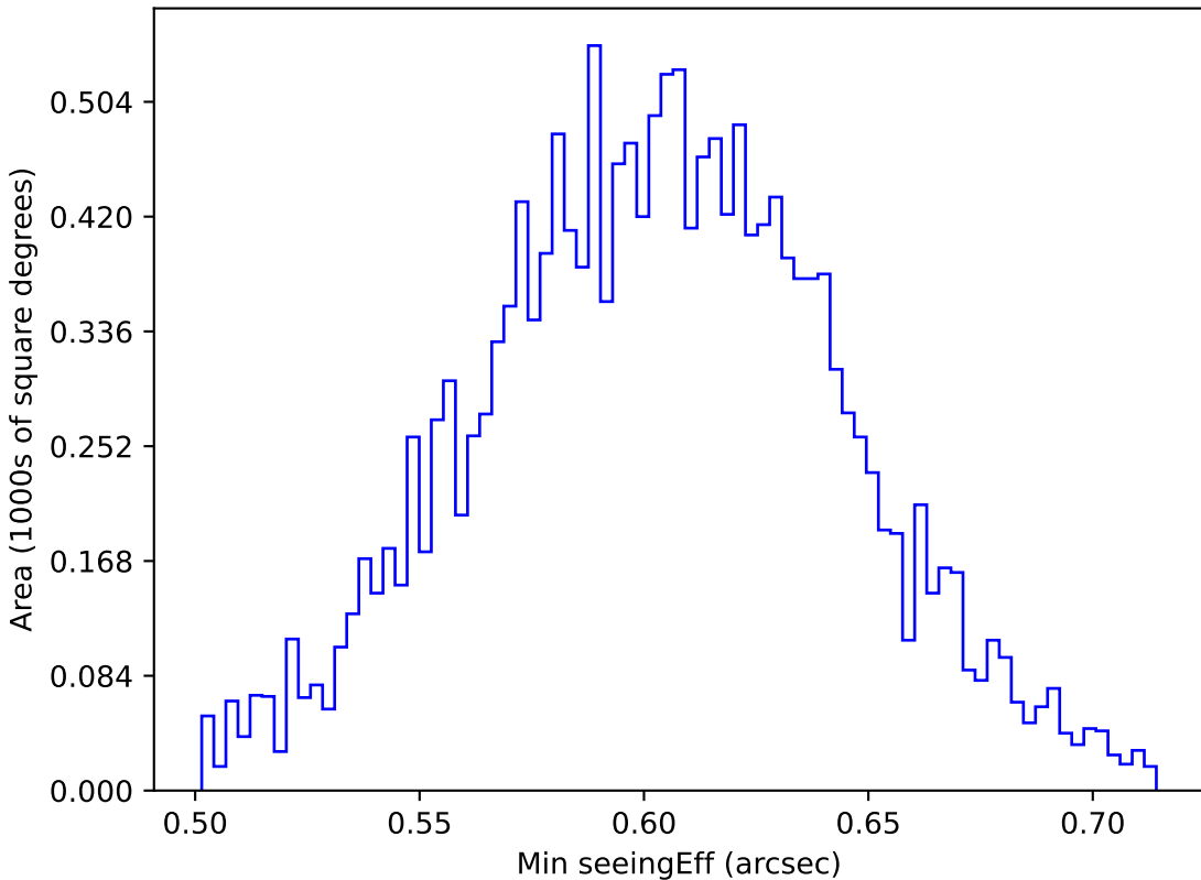
too_ignore_100_1v3.4_10yrs WFD i band: Min seeingEff
