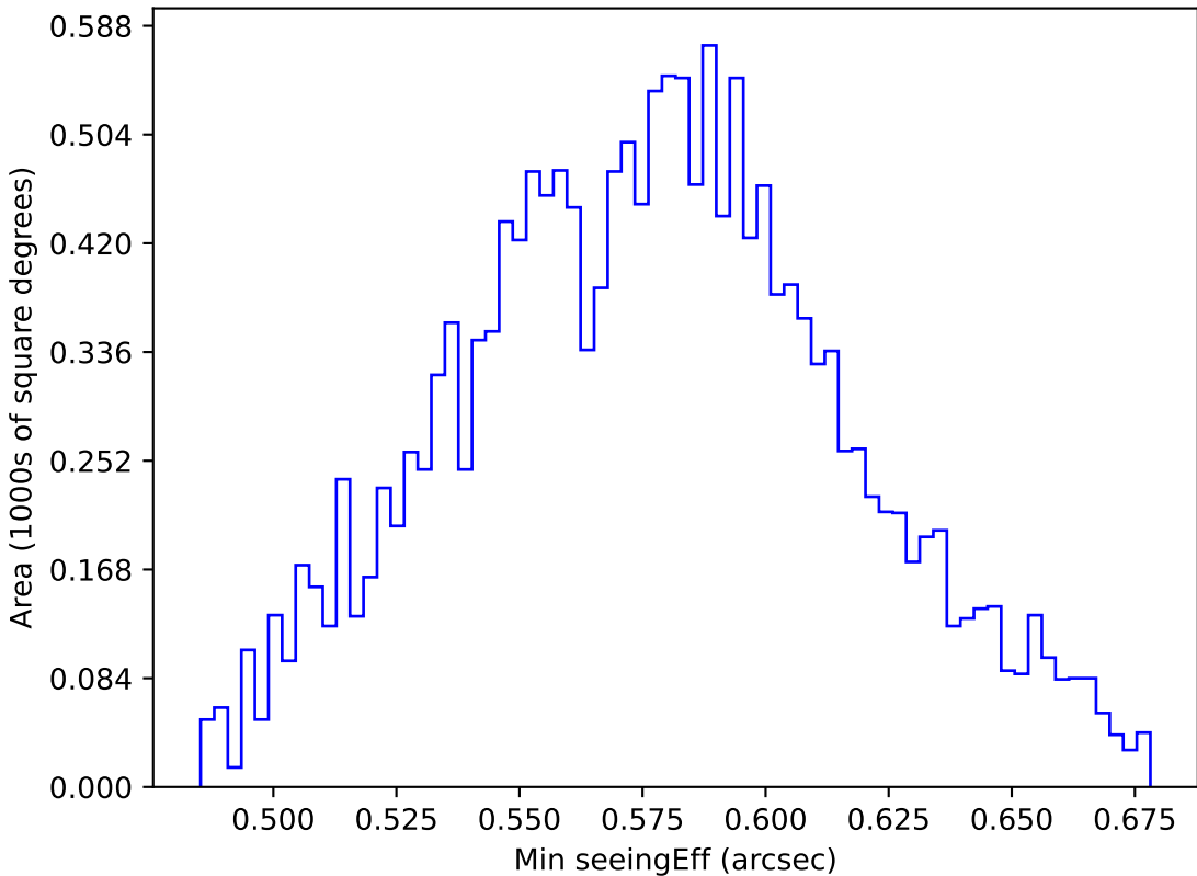
too_ignore_100_1v3.4_10yrs WFD all bands: Min seeingEff
