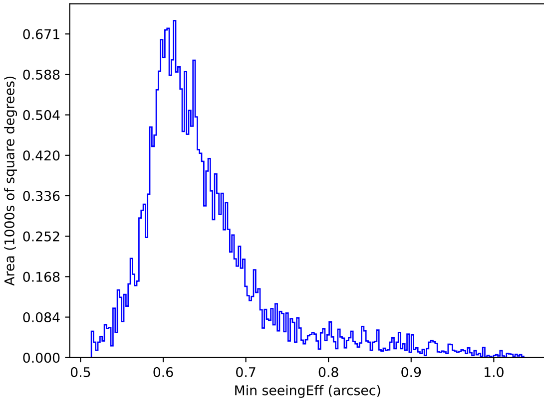
too_ignore_100_1v3.4_10yrs All sky z band: Min seeingEff
